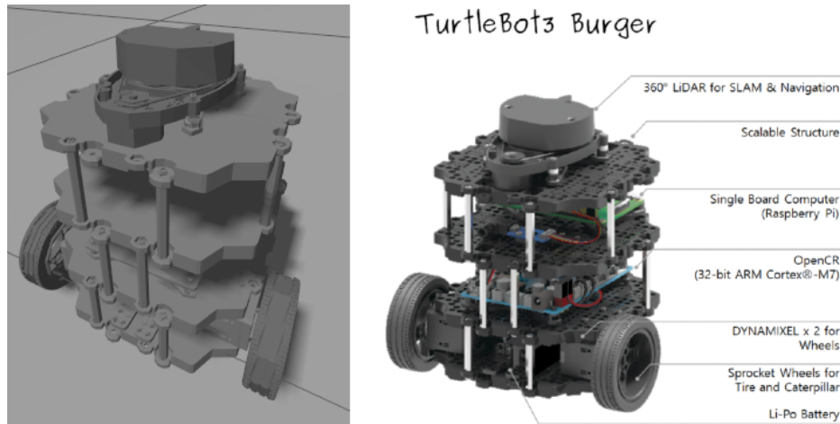
Figure 1: The turtlebot robot and its simulation in Gazebo.
